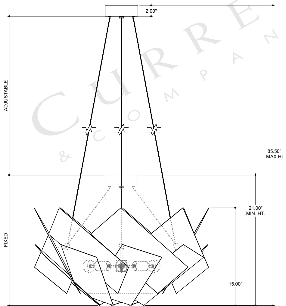
FRONT VIEW
