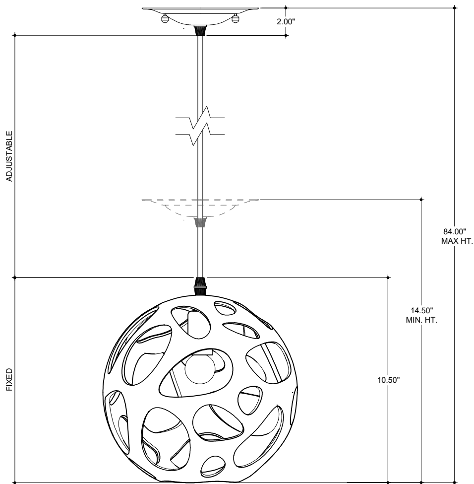
FRONT VIEW
