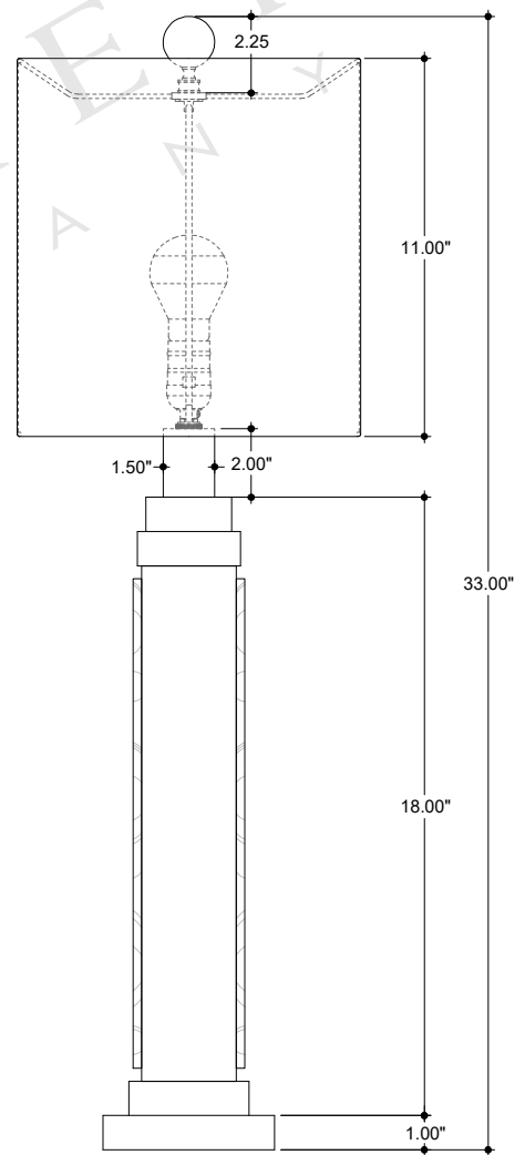
SIDE VIEW
