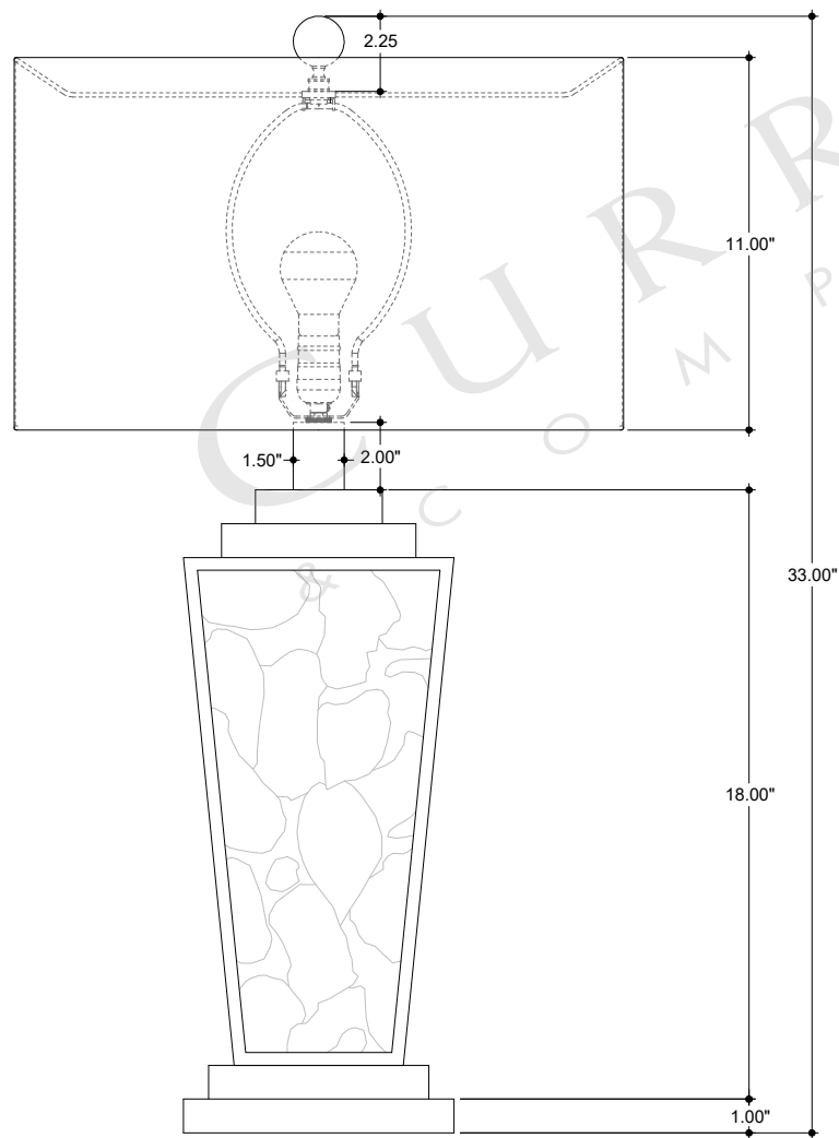
FRONT VIEW
