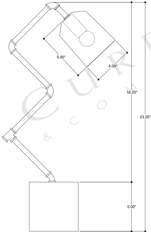
FRONT VIEW
