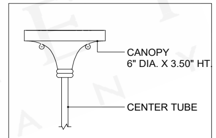
CANOPY DETAIL
