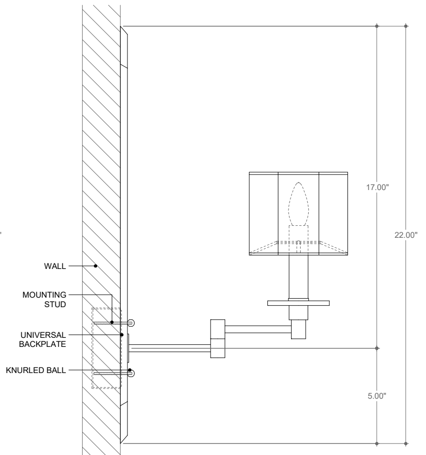
SIDE VIEW
