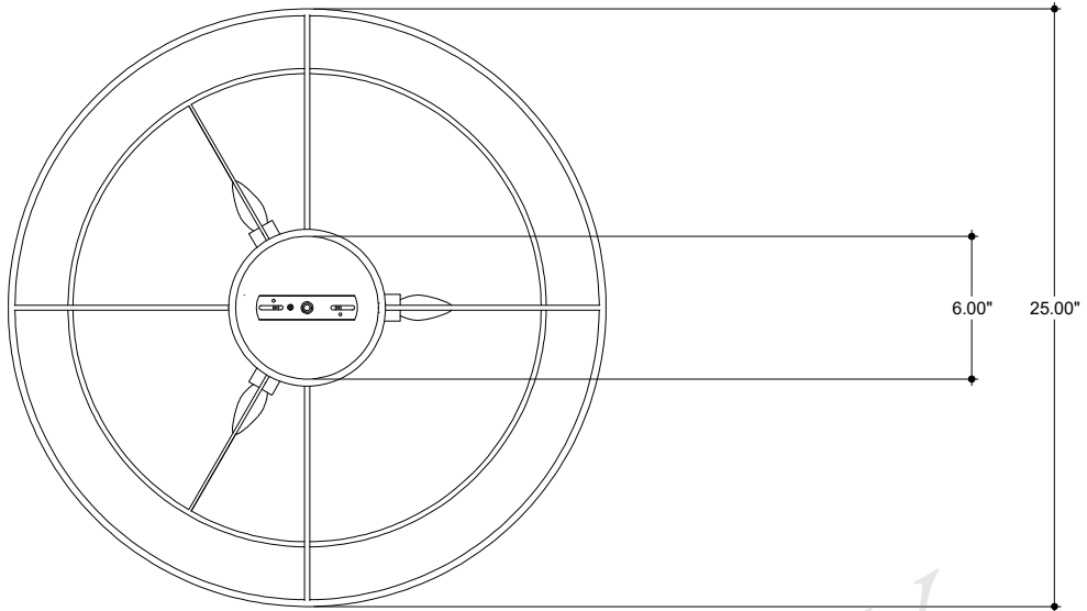
TOP VIEW
