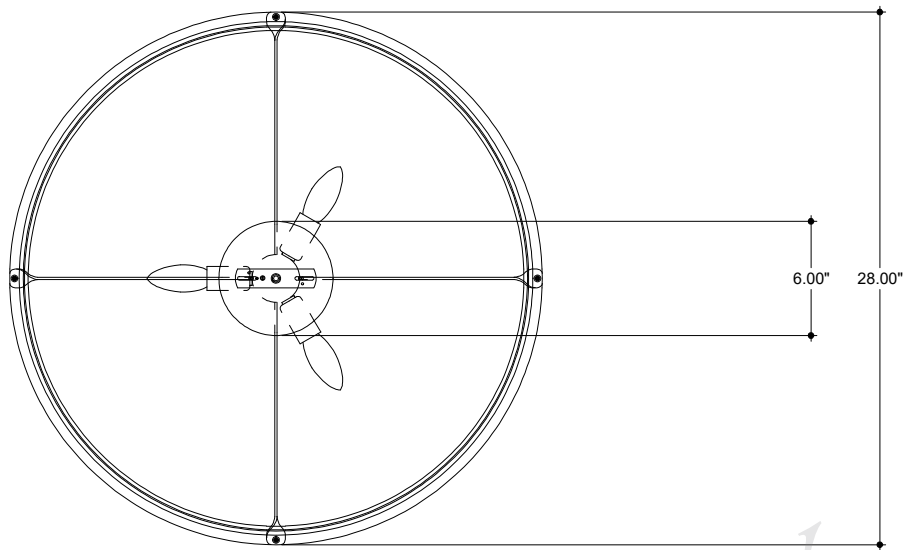
TOP VIEW
