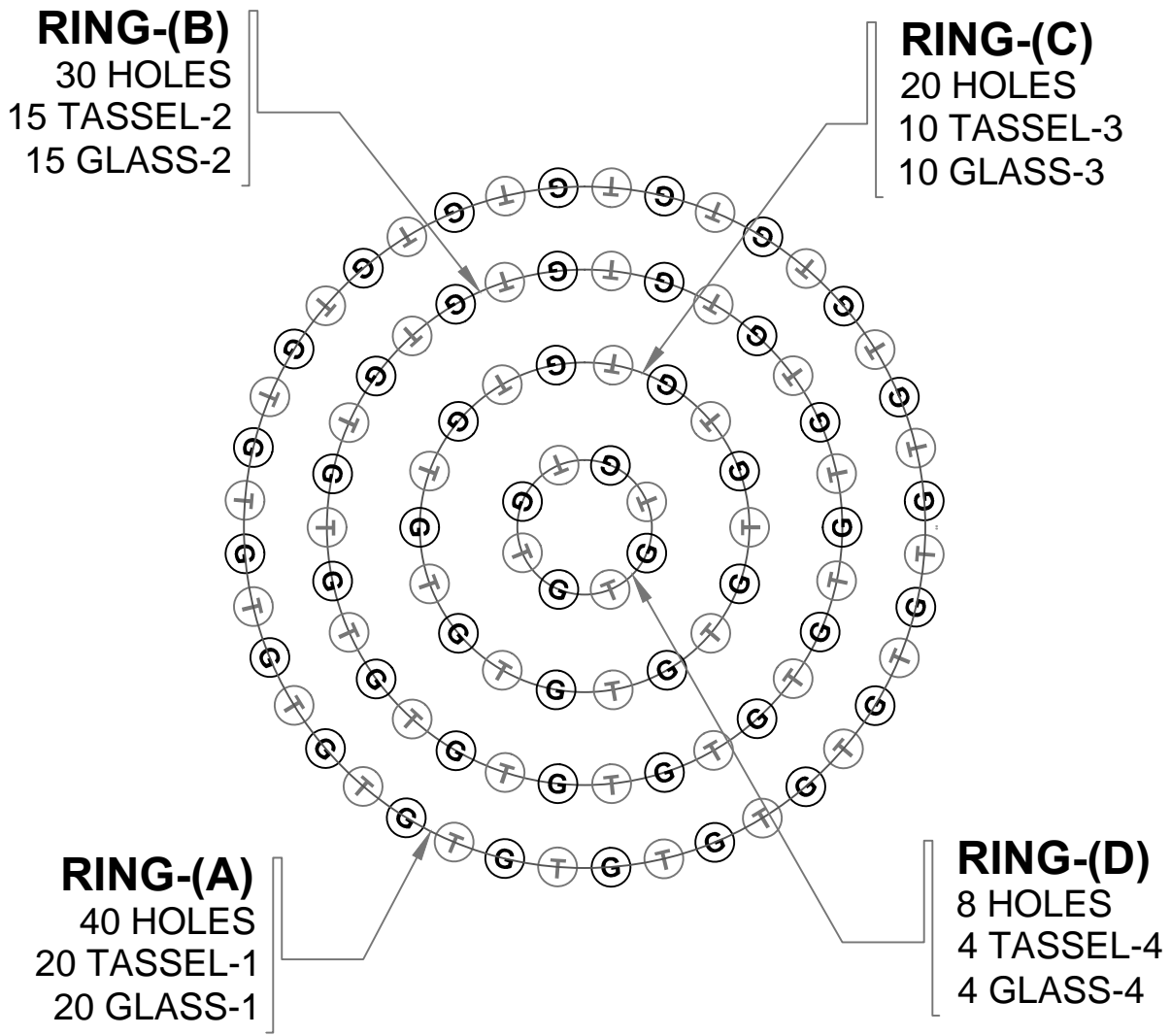
PLAN VIEW
