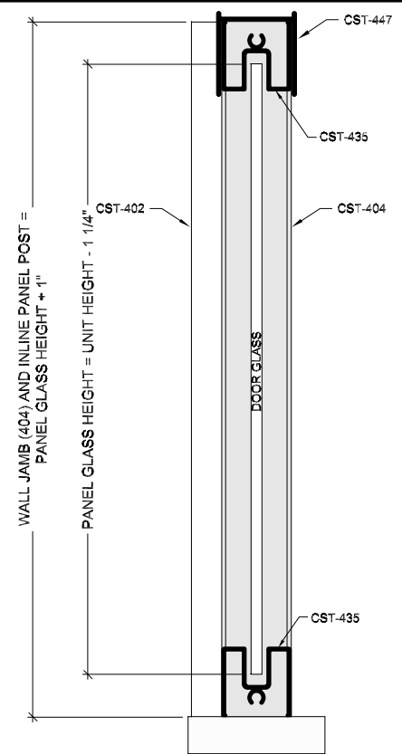
Neo Wing Panel vertical cross section
