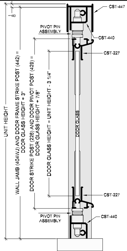
Neo Legend Door vertical cross section
