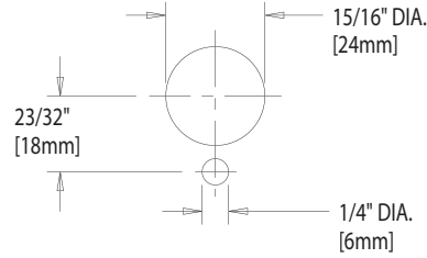
PLAN VIEW HOLE LOCATION FOR BODY SHANK AND PIN
