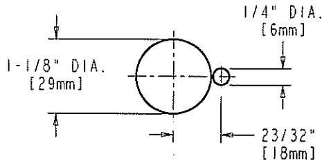
PLAN VIEW HOLE LOCATION FOR BODY SHANK AND PIN
