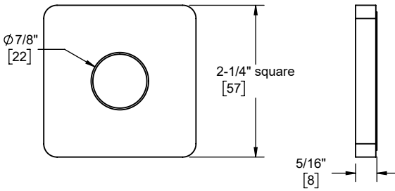
9130-65
