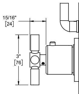
TO-THF1L-30X side view
