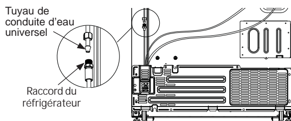
Tuyau 1/4 po
