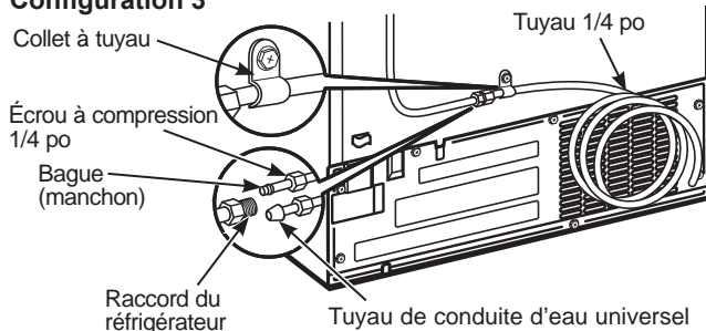
Tuyau 1/4 po
