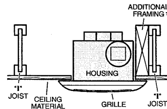
HOUSING MOUNTED TO "I" JOIST Requires additional framing for mounting. Discharge parallel to joists.
