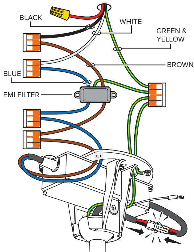
Wiring Diagram (With EMI Filter)
