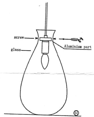
H. Fasten the glass and the aluminium part by screw. (Do not fasten the screw too tight, otherwise the glass will break.)
