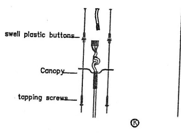
K. Install the swell plastic buttons into the ceiling. Use the tapping screws to fix the bracket into the ceiling. L. Connect the power wire to the terminal block. M. Fix the canopy to the bracket by screws.
