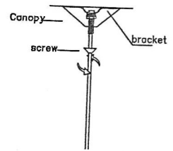
K. Install the swell plastic buttons into the ceiling. Use the tapping screws to fix the bracket into the ceiling. L. Connect the power wire to the terminal block. M. Fix the canopy to the bracket by screws.
