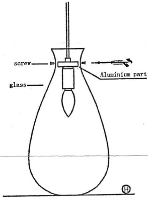
H. Fasten the glass and the aluminium part by screw. (Do not fasten the screw too tight, otherwise the glass will break.)
