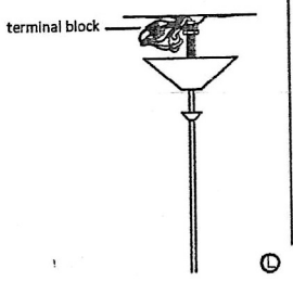
L. Connect the power wire to the terminal block.
