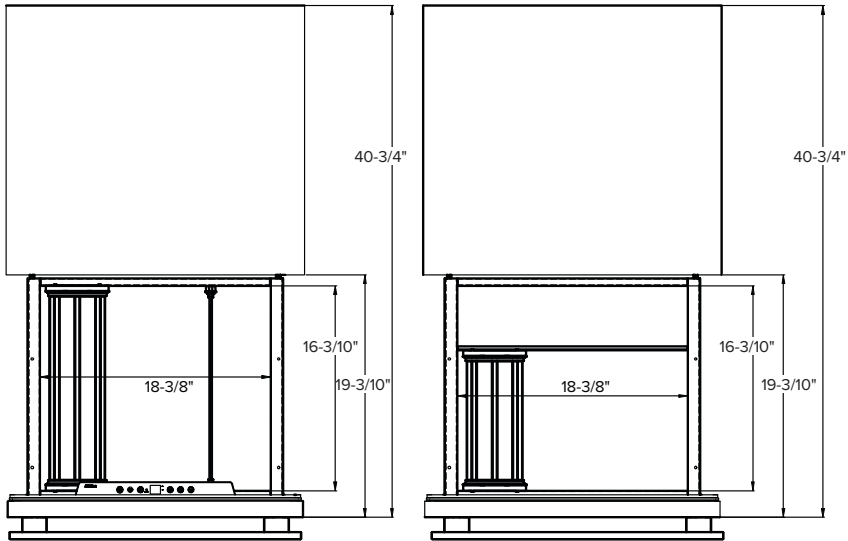
Undercounter Dimensions
