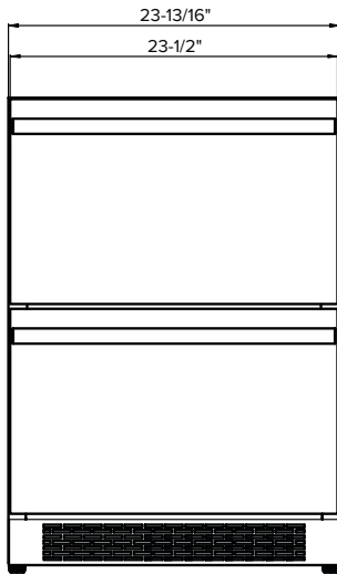
Undercounter Dimensions
