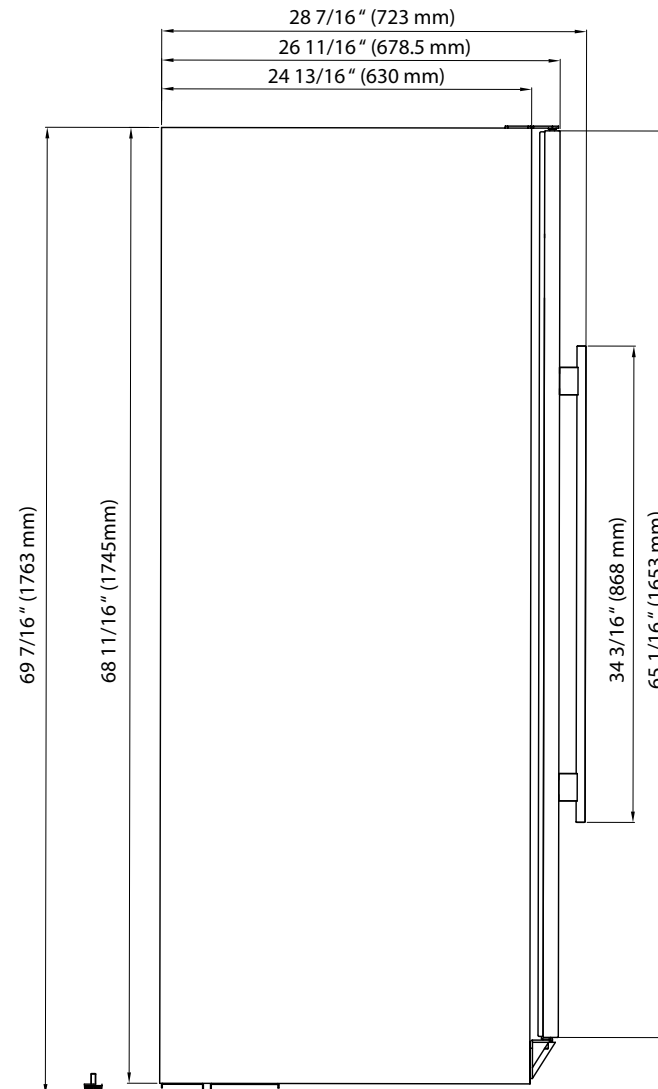
Side View
