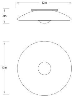
DFC37 STELLA FLUSH MOUNT
