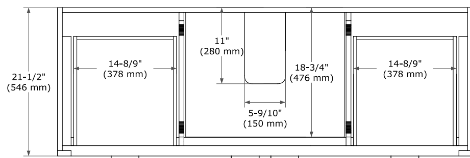
PLAN VIEW
