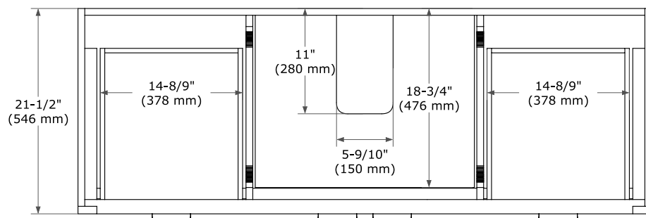
PLAN VIEW
