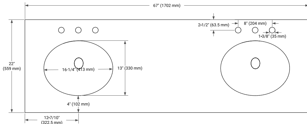
COUNTERTOP PLAN VIEW
