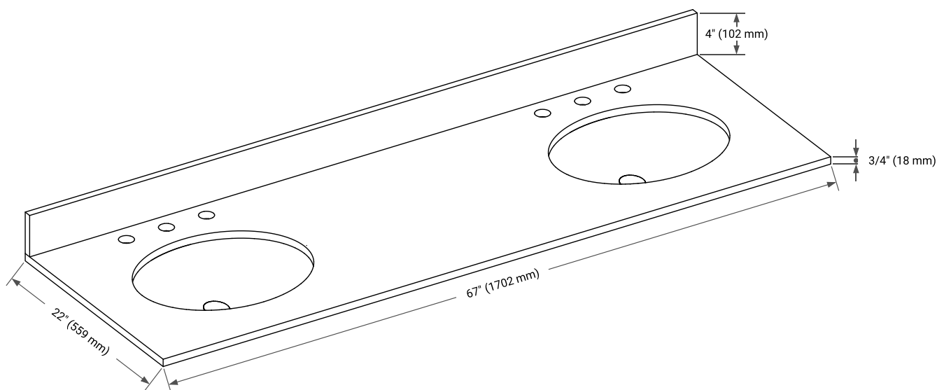
THREE DIMENSIONAL COUNTERTOP VIEW
