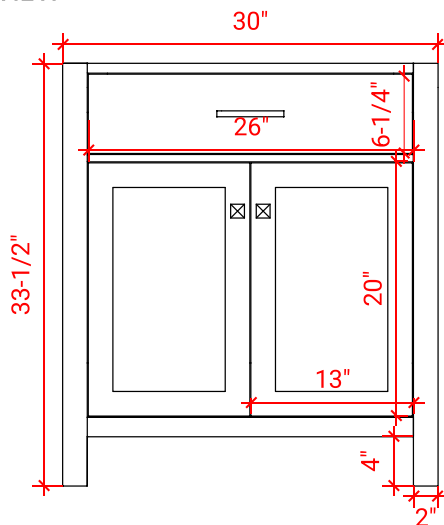
PLAN VIEW
