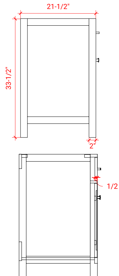
SIDE VIEW
