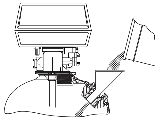
FILLING MEDIA TANK
