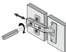
HORIZONTAL ADJUSTMENT To move the door left or right.
