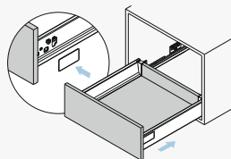
Roll in the drawer
