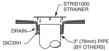
SECTION THRU DRAIN CONNECTION
