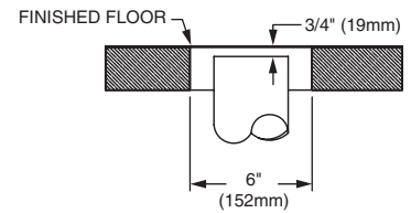
SUGGESTED INSTALLATION THRU DRAIN PIPE
