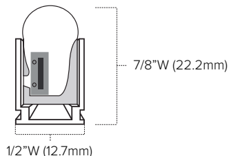
Cut-view when used with MINI-P2-NF-CHAN-3 (sold separately)
