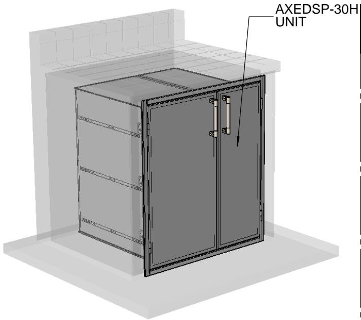
AXEDSP-30H TYPICAL INSTALLATION
