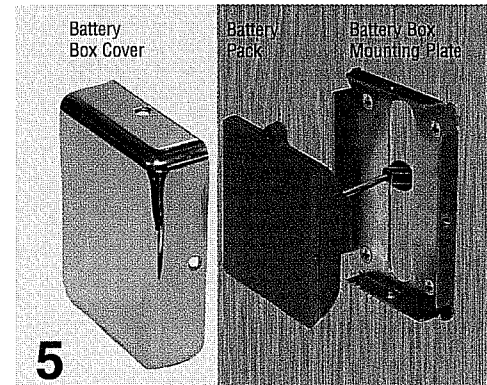
5. Connect battery pack and place inside of battery mounting plate. Position cover and fasten with three #6-32 x 5/16" screws.
