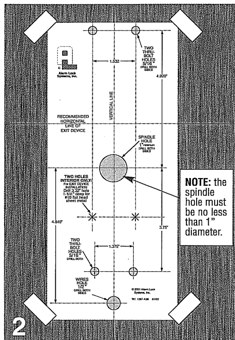
2. Existing Installation: Position Alarm Lock template on horizontal & vertical lines of existing spindle hole. New Installation: Locate and mark horizontal and vertical lines indicated in Exit Device Instructions/Template. Line up Alarm Lock template with horizontal and vertical lines and tape on door. Existing and New Installations: Mark all hole centers on each side of door. Drill all holes from both sides of door to avoid splintering.
