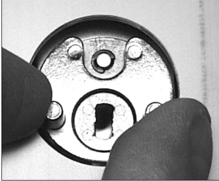
Fig. 7: Position the interface cylinder
