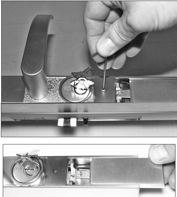
Fig. 10: Loosen battery cover screw only until the battery cover is able to slide off
