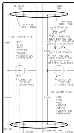
Fig. 4: Template (WI1459) through-bolt holes (circled)
