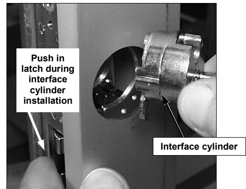
Fig. 6a: Push latch in and hold
