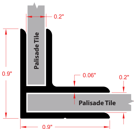
Cross-Section
