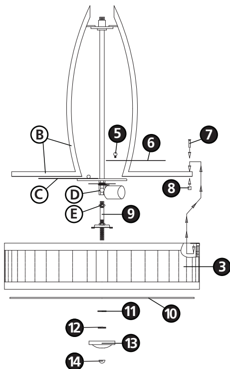
Drawing 2 - Fixture Assembly
