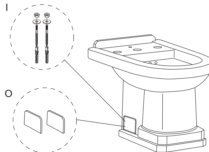
Bidet Cirtangular™ DC024110
