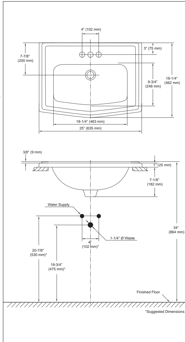
LT781.4 Baldwin Self-Rimming Lavatory
