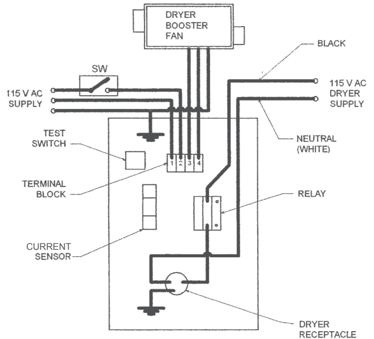
INSTALLATION CONNECTIONS
