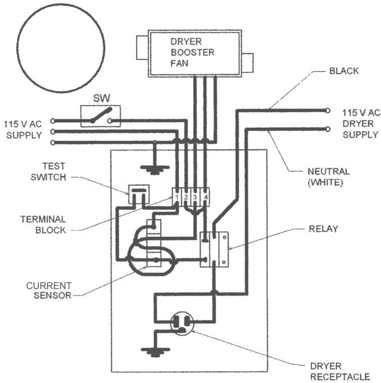
SCHEMATIC WIRING DIAGRAM
