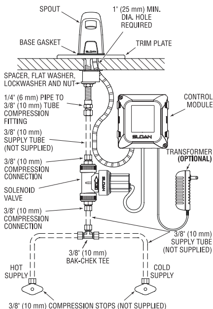
EBF-625 Faucet with Bak-Chek ® Tee for Hot and Cold Water Supply (shown with 4" trim plate)
