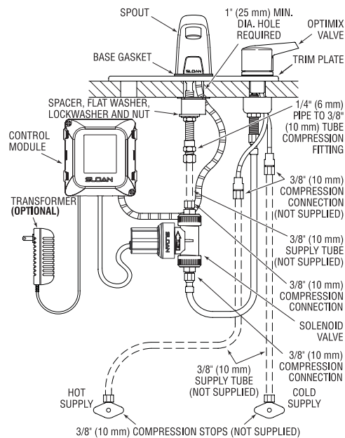
EBF-625 Faucet with ADM Variation Mixing Valve for Hot and Cold Water Supply (shown with 8" trim plate)
