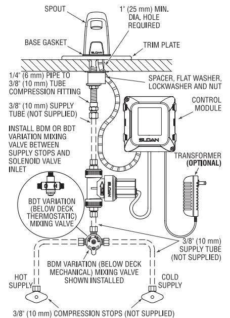
EBF-625 Faucet with BDM and BDT Variation Mixing Valves for Hot and Cold Water Supply (shown with 4" trim plate)
