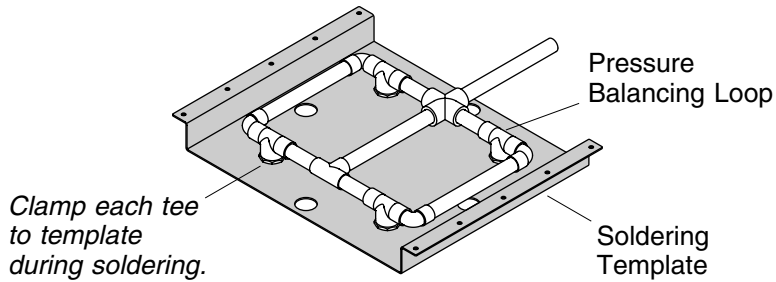
Soldering Template
