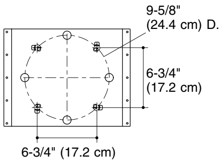
Soldering Template
