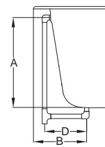
Drain/Overflow
