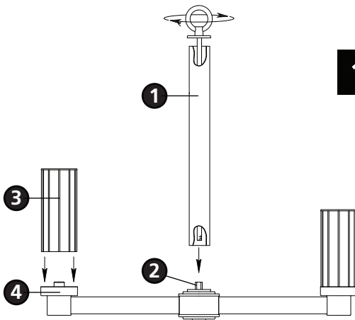
Drawing 1 - Fixture Assembly
