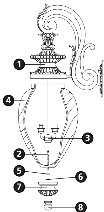
Drawing 3 - Fixture Assembly
