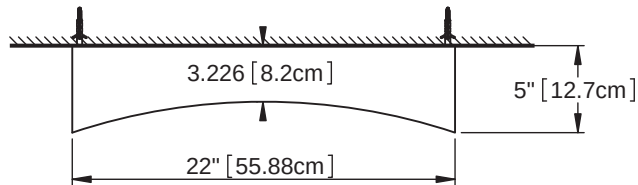
Top View
