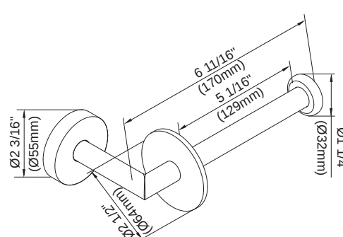
Single Post Paper Holder
