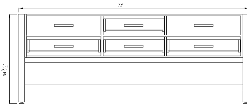
FRONT
