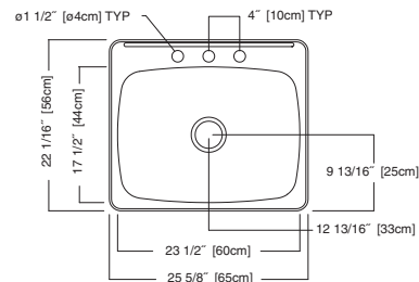
21SB.252283.073 Standard drilling: 3 hole
