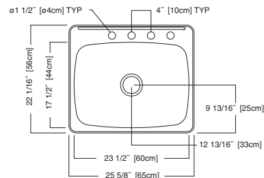
21SB.252284.073 Optional drilling: 4th hole on right
