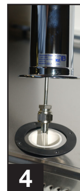
Thread beer line connector to draft arm and secure draft arm to cabinet with rubber gasket under the draft arm.
