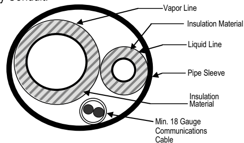
Figure 70: Typical Arrangement of Refrigerant Pipe and Cable(s) in a Utility Conduit.
